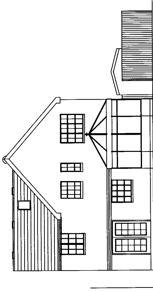
Rear Elevation
